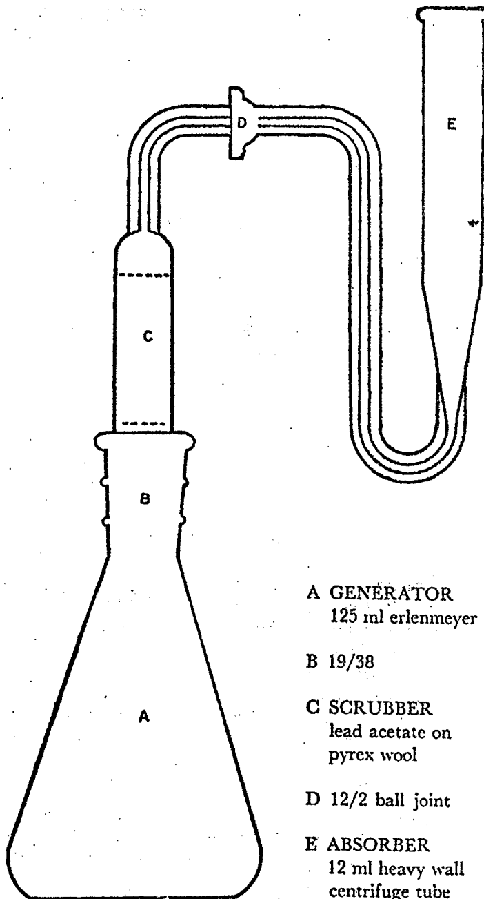
Figure 1 — Arsine Generator
