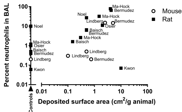
Fig. 8. Data from the literature illustrating BAL neutrophil percentage as function of deposited \text{TiO}_2 surface area in the lungs. Data from studies described in Table 3 are presented in graphical form. Percentage neutrophils in BAL were assessed either immediately after exposure or up to 24 h after exposure as detailed in Table 3. The name of the first author of the used reference is added as a label of each data point. Some data from refs (32,57) are not depicted because the percentage of neutrophils was zero, and only values higher than zero can be plotted on the logarithmic y scale.
