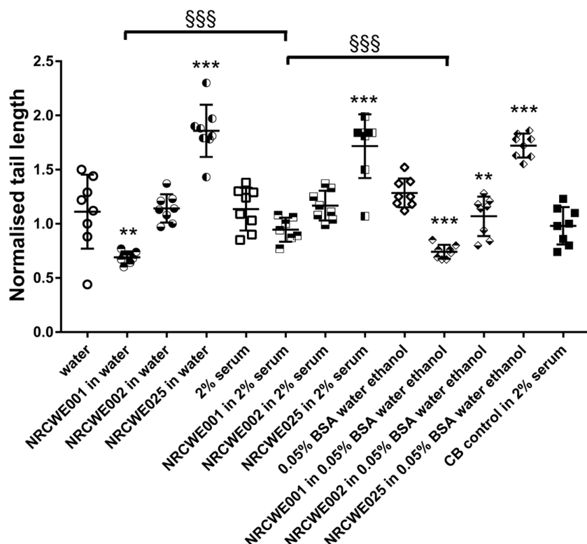
Fig. 7. DNA strand break levels in BAL cells 24 h after pulmonary exposure to \text{TiO}_2 and CB in mice. Three different \text{TiO}_2 were administered intratracheally to mice at 67 \mu\text{g}/\text{mouse} . CB was administered at 162 \mu\text{g}/\text{mouse} . Twenty-four hours later BAL fluid was prepared, and tail length was measured by comet assay. Data are mean and bars represent SD. ***, ** and * designates P -values of <0.001 , <0.01 and <0.05 , respectively, of one-way ANOVA with Holm-Sidak's multiple comparisons test of \text{TiO}_2 particles against dispersion medium in case of data approaching normality and not having a highly different variation (details given in the Methods section), otherwise of Kruskal-Wallis test with Dunn's multiple comparisons test. $$$, $$ and $ designate P -values of <0.001 , <0.01 and <0.05 , respectively, of \text{TiO}_2 data of each \text{TiO}_2 particle type against each other of one-way ANOVA with Holm-Sidak's multiple comparisons test in case of data approaching normality and not having a highly different variation (details given in the Methods section), otherwise of Kruskal-Wallis test with Dunn's multiple comparisons test.
